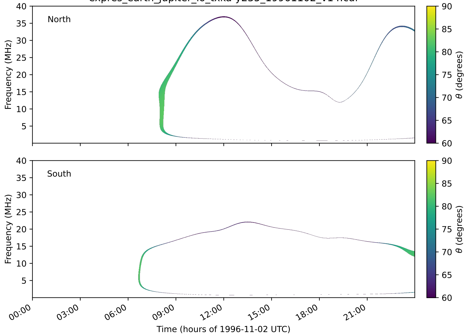
expres_earth_jupiter_io_txka-y235_19961102_v14.cdf
