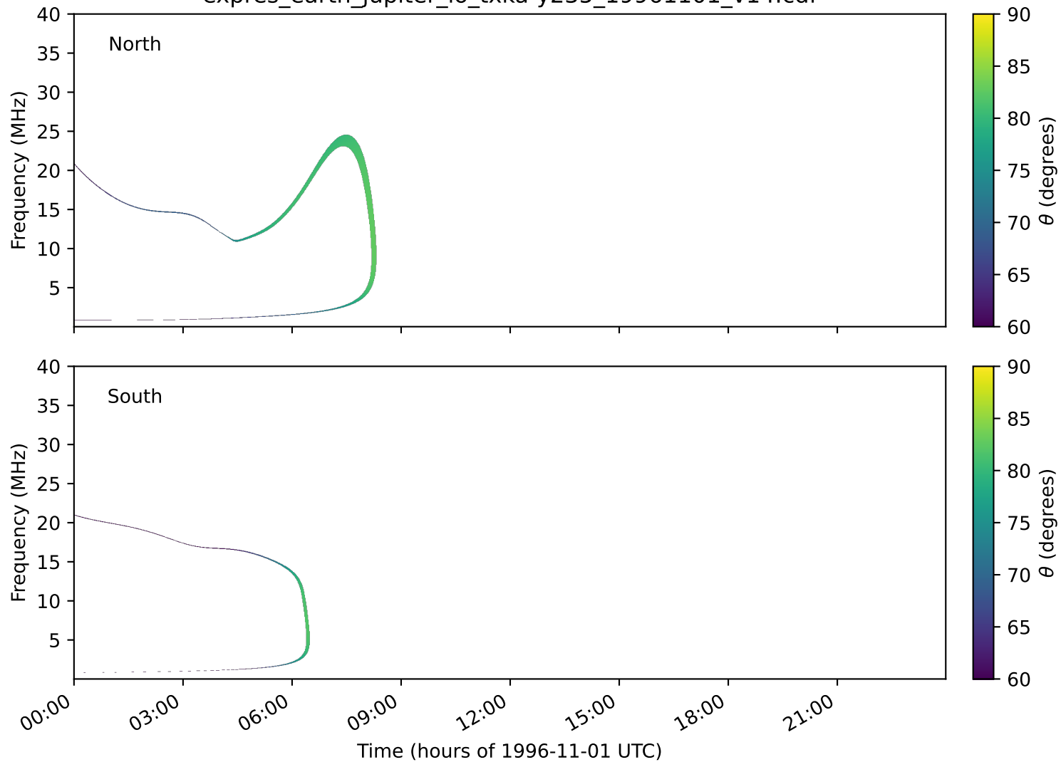
expres_earth_jupiter_io_txka-y235_19961101_v14.cdf
