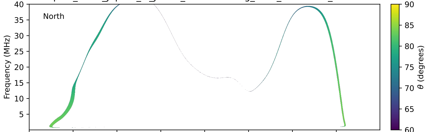
expres_earth_jupiter_io_jrm33_lossc-wid1deg_3kev_19961127_v11.cdf
