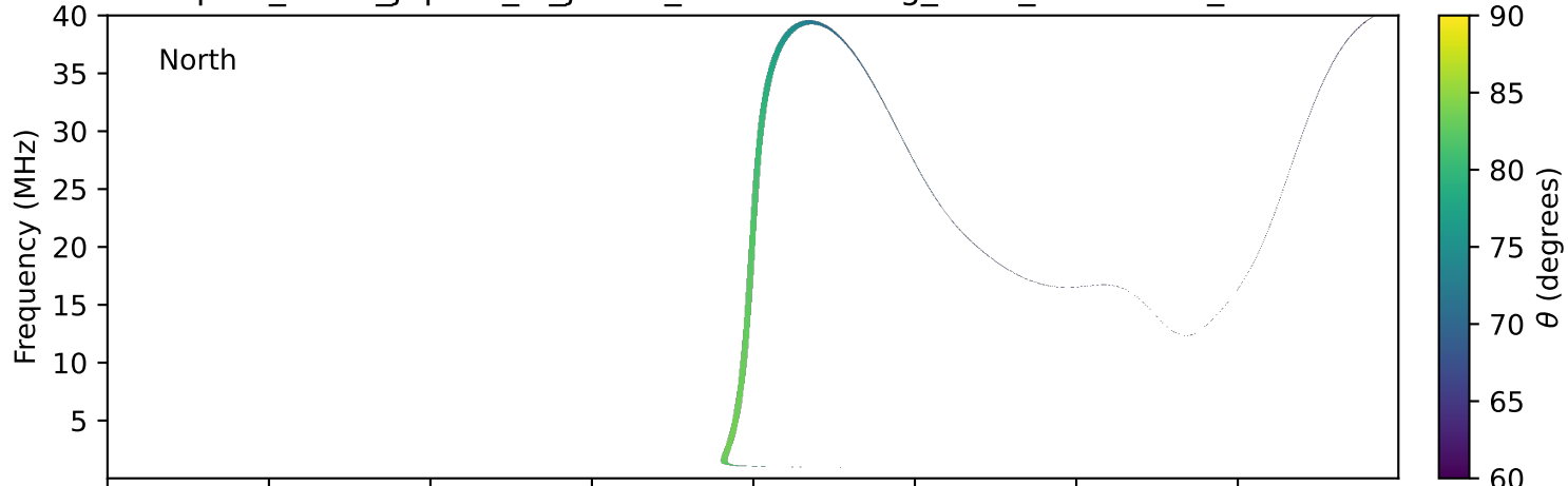
expres_earth_jupiter_io_jrm33_lossc-wid1deg_3kev_19961116_v11.cdf
