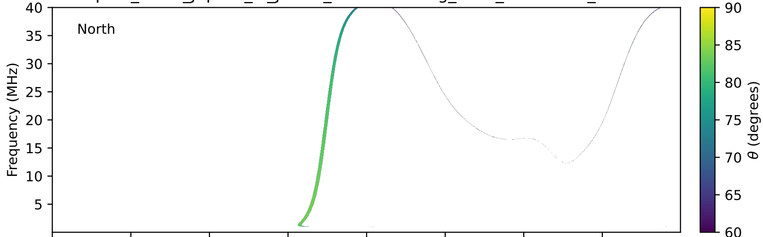
expres_earth_jupiter_io_jrm33_lossc-wid1deg_3kev_19961109_v11.cdf
