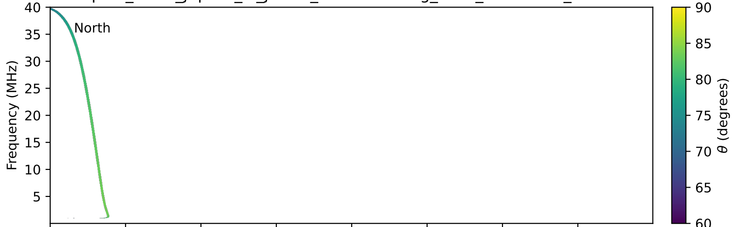
expres_earth_jupiter_io_jrm33_lossc-wid1deg_3kev_19961103_v11.cdf
