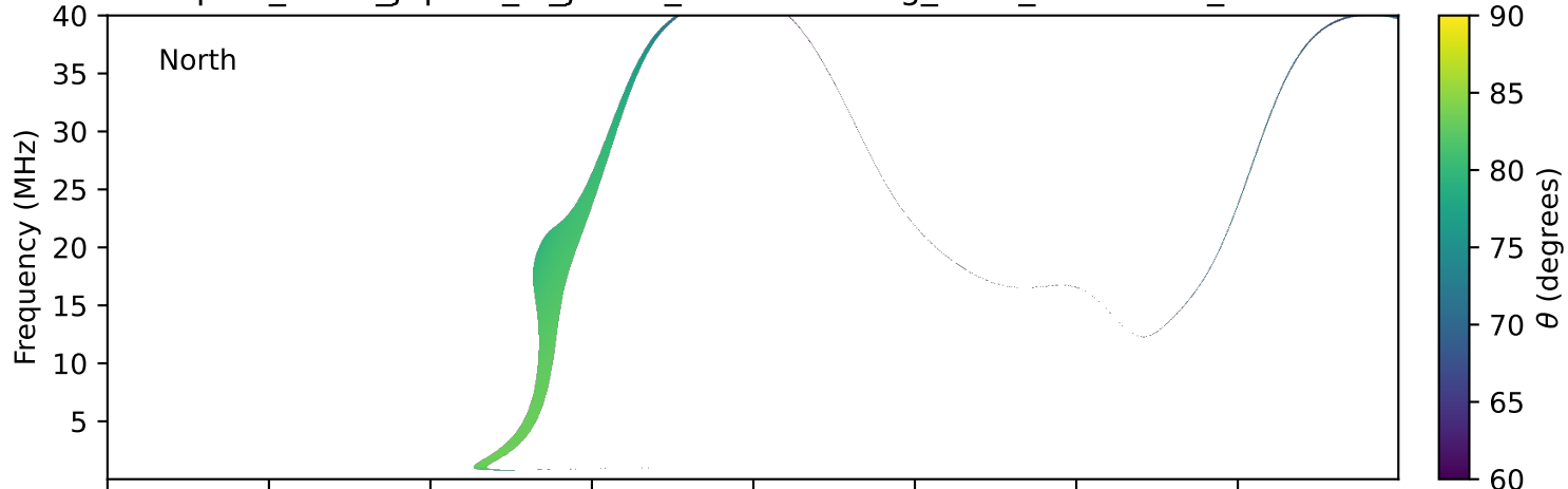
expres_earth_jupiter_io_jrm33_lossc-wid1deg_3kev_19961102_v11.cdf
