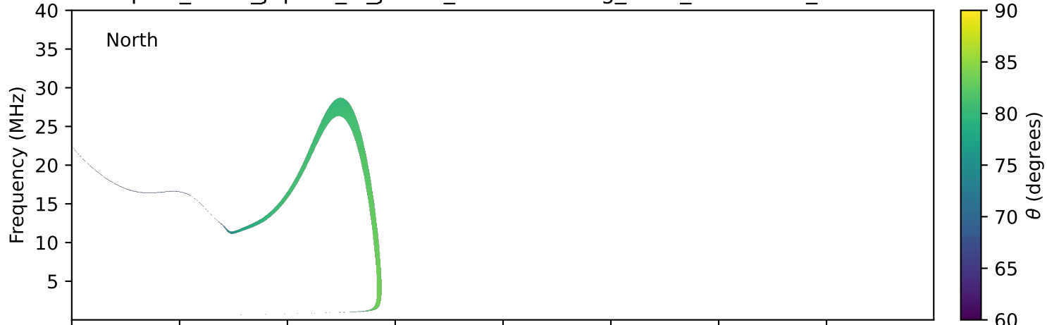
expres_earth_jupiter_io_jrm33_lossc-wid1deg_3kev_19961101_v11.cdf
