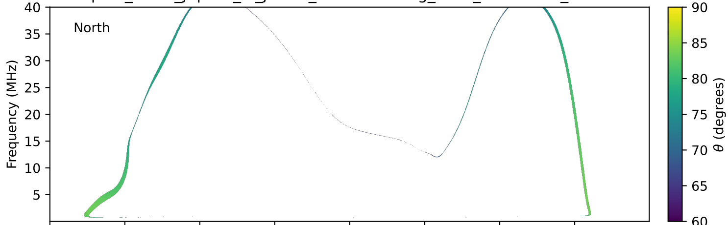
expres_earth_jupiter_io_jrm09_lossc-wid1deg_3kev_19961127_v11.cdf
