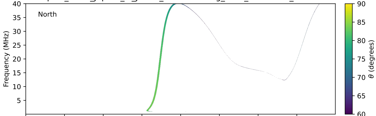
expres_earth_jupiter_io_jrm09_lossc-wid1deg_3kev_19961109_v11.cdf
