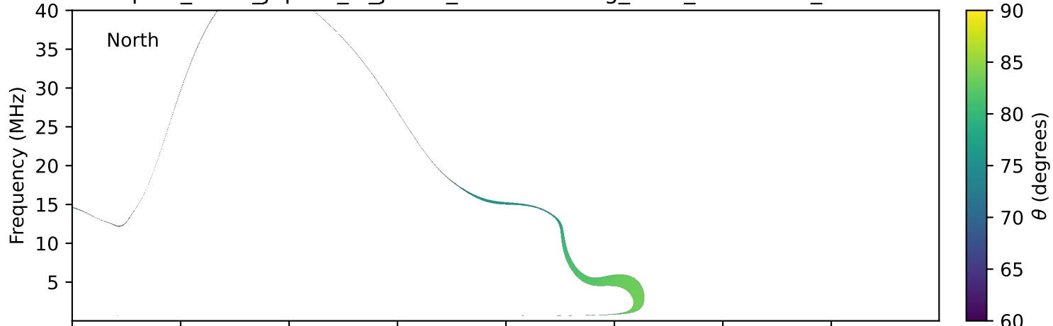
expres_earth_jupiter_io_jrm09_lossc-wid1deg_3kev_19961106_v11.cdf
