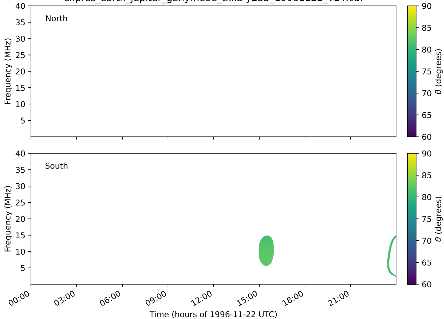
expres_earth_jupiter_ganymede_txka-y235_19961122_v14.cdf
