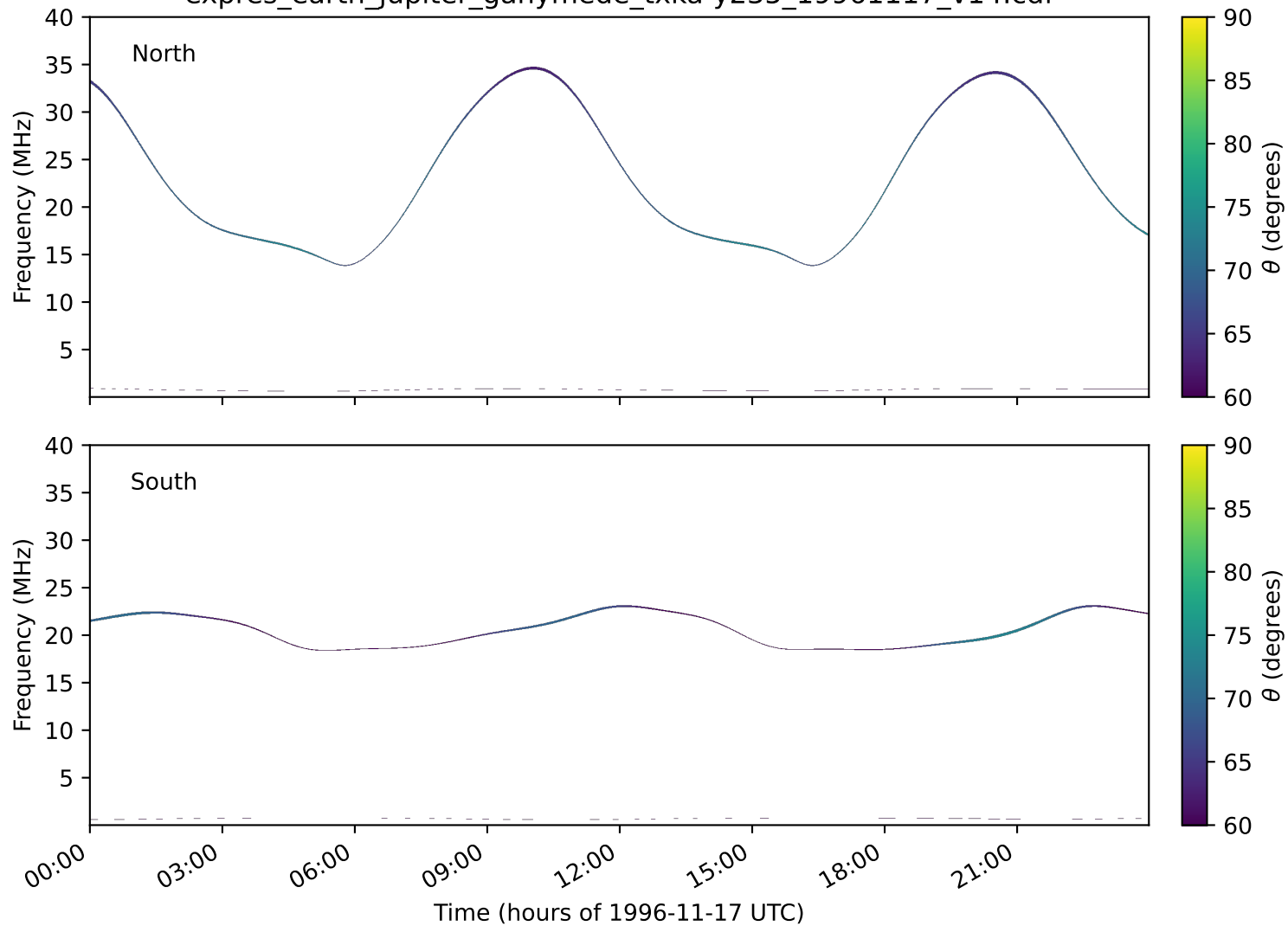
expres_earth_jupiter_ganymede_txka-y235_19961117_v14.cdf
