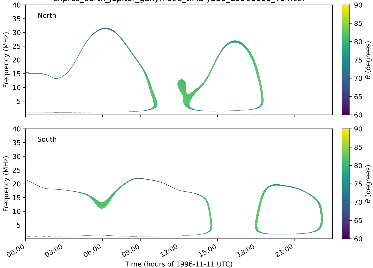
expres_earth_jupiter_ganymede_txka-y235_19961111_v14.cdf
