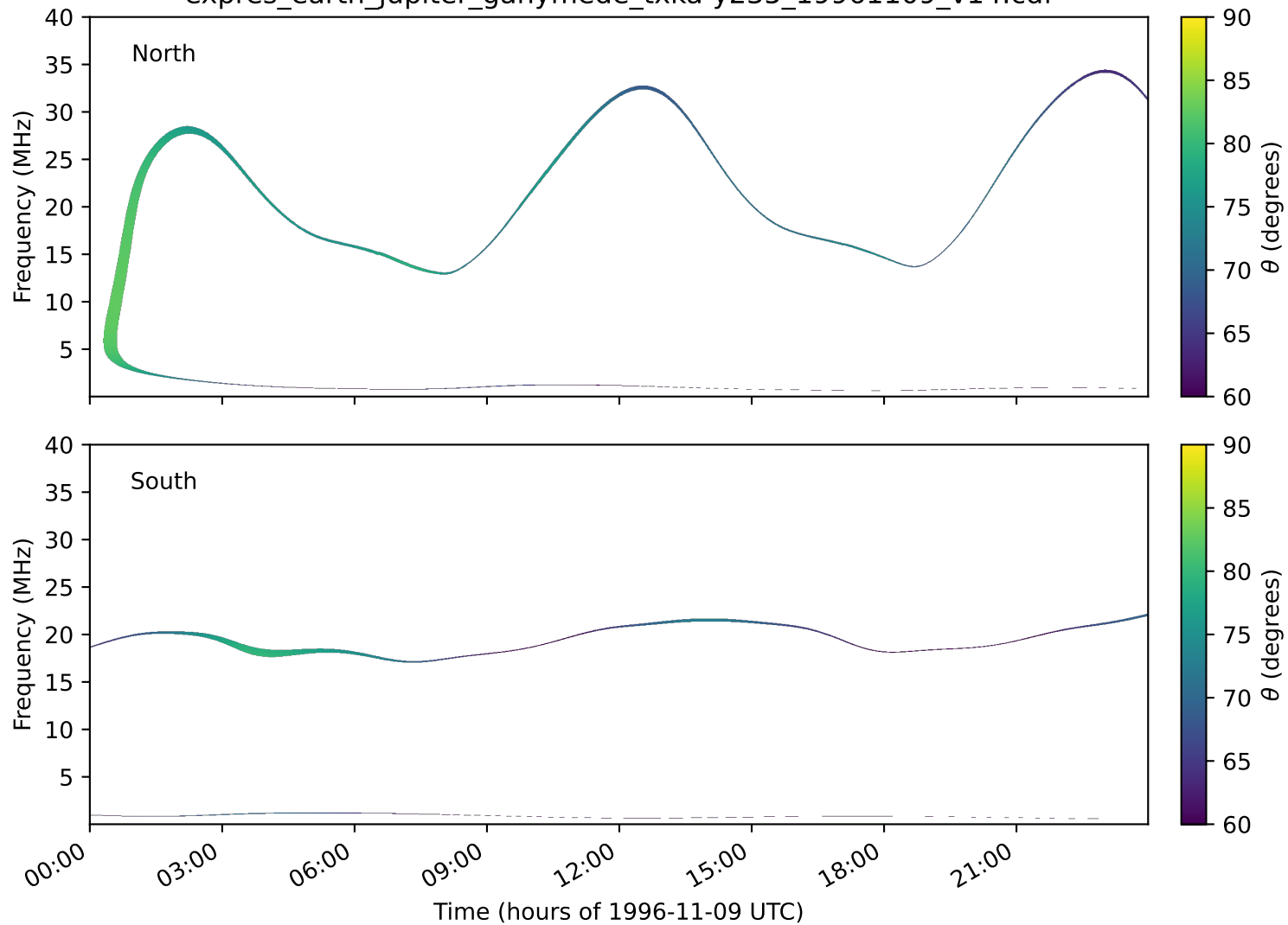
expres_earth_jupiter_ganymede_txka-y235_19961109_v14.cdf
