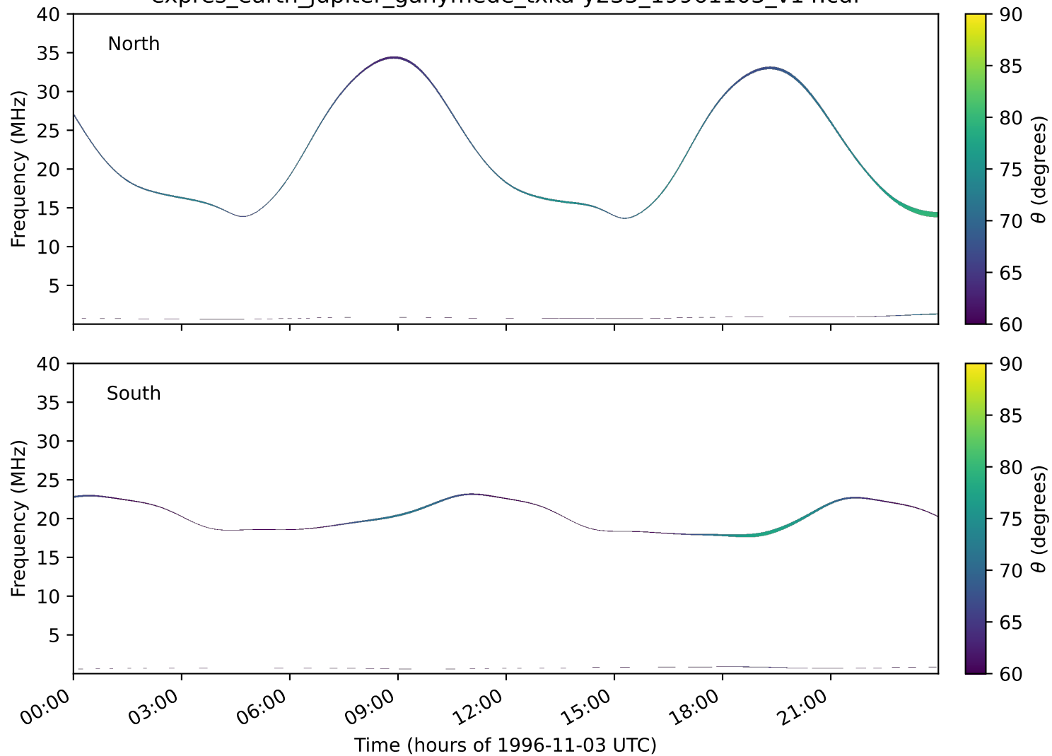
expres_earth_jupiter_ganymede_txka-y235_19961103_v14.cdf
