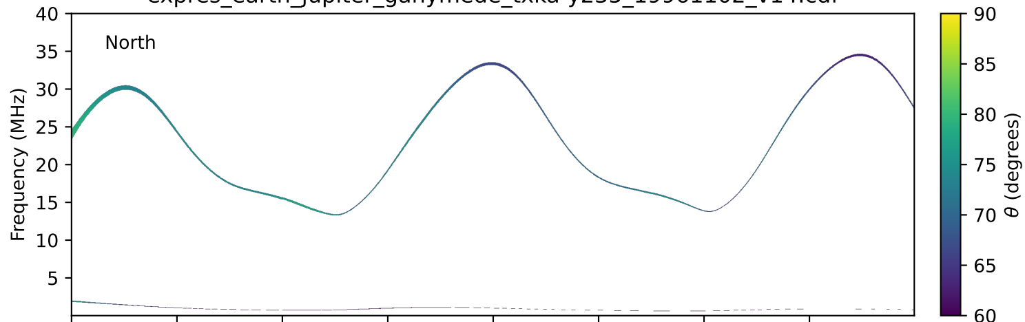
expres_earth_jupiter_ganymede_txka-y235_19961102_v14.cdf
