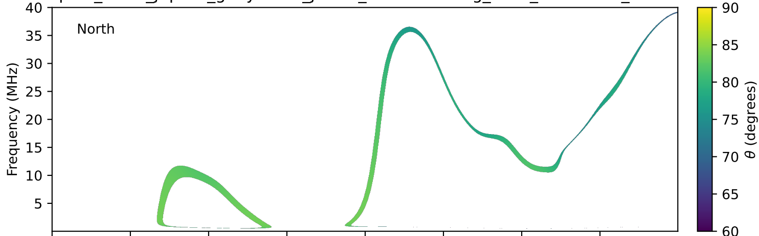
expres_earth_jupiter_ganymede_jrm33_lossc-wid1deg_3kev_19961123_v11.cdf
