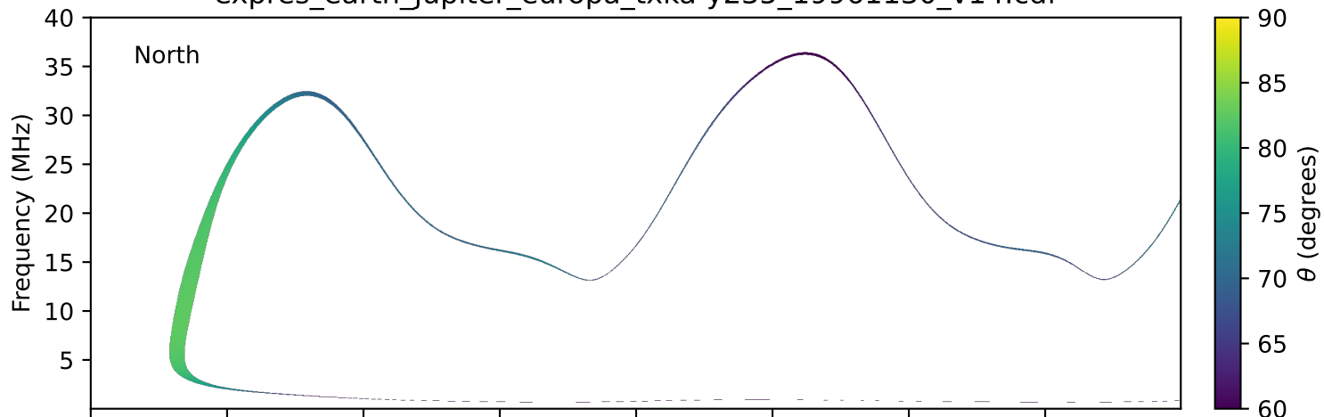
expres_earth_jupiter_europa_txka-y235_19961130_v14.cdf
