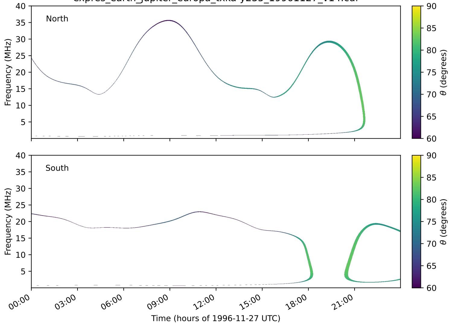
expres_earth_jupiter_europa_txka-y235_19961127_v14.cdf
