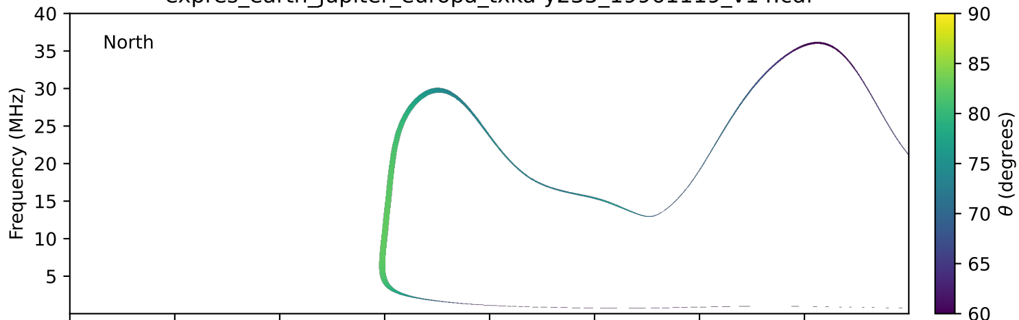
expres_earth_jupiter_europa_txka-y235_19961119_v14.cdf
