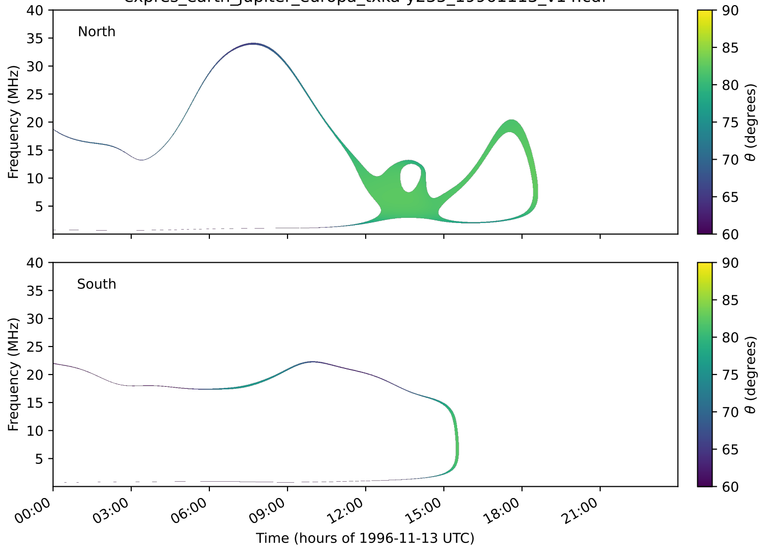
expres_earth_jupiter_europa_txka-y235_19961113_v14.cdf
