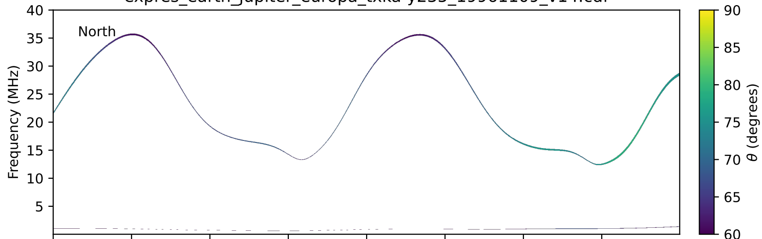
expres_earth_jupiter_europa_txka-y235_19961109_v14.cdf
