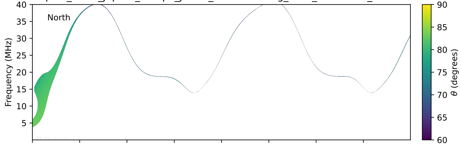
expres_earth_jupiter_europa_jrm33_lossc-wid1deg_3kev_19961123_v11.cdf
