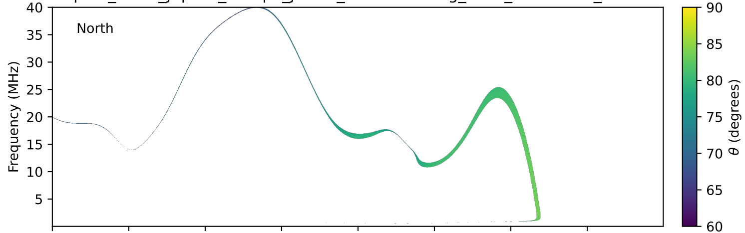
expres_earth_jupiter_europa_jrm33_lossc-wid1deg_3kev_19961113_v11.cdf
