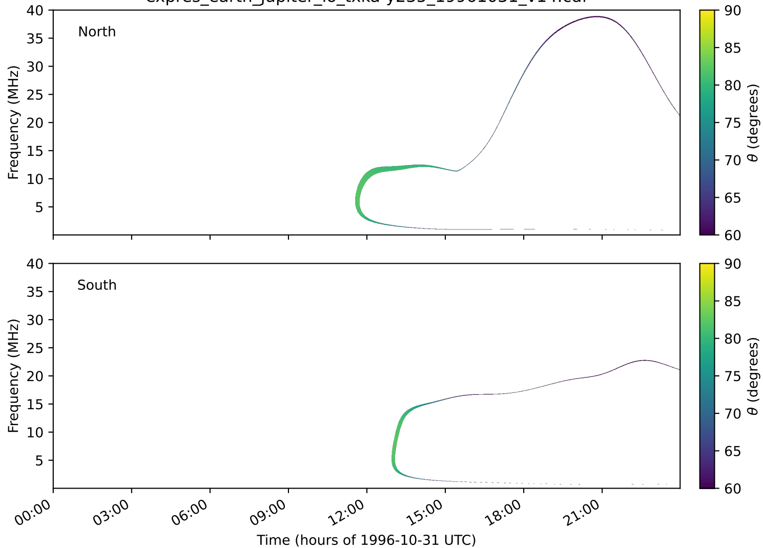
expres_earth_jupiter_io_txka-y235_19961031_v14.cdf
