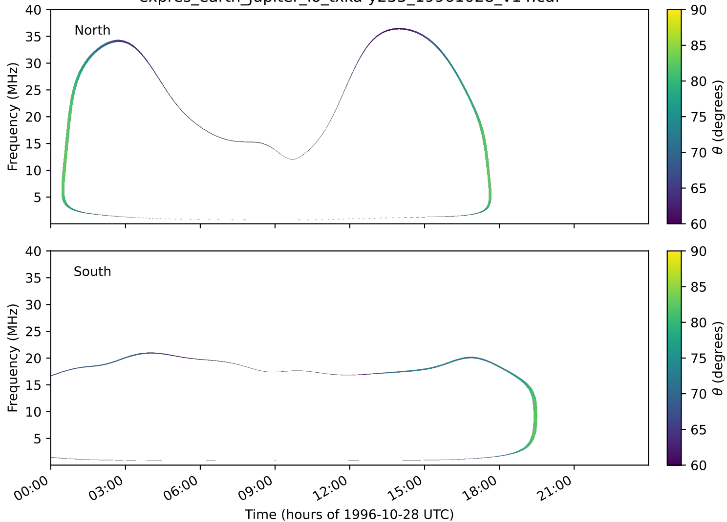
expres_earth_jupiter_io_txka-y235_19961028_v14.cdf
