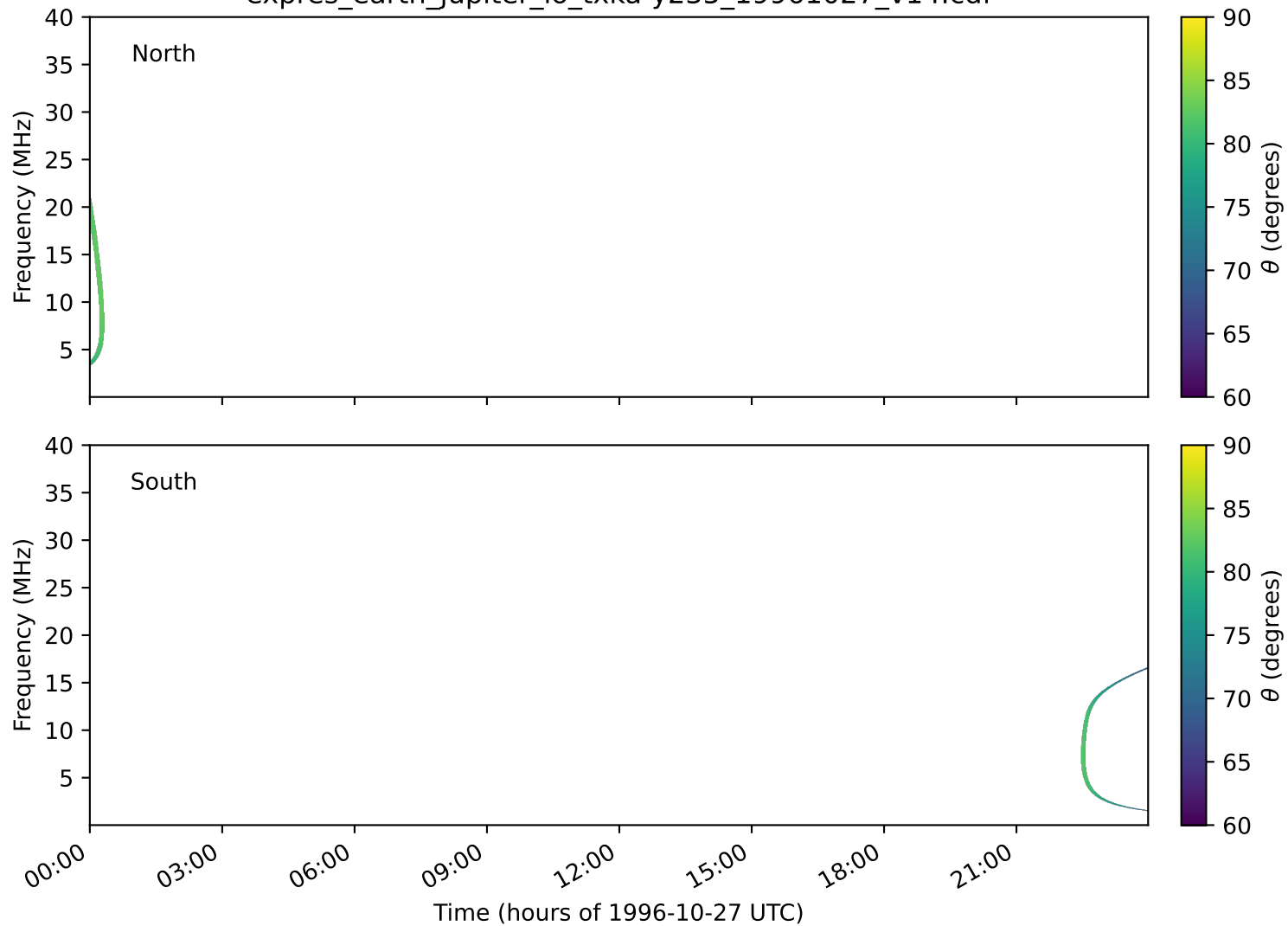
expres_earth_jupiter_io_txka-y235_19961027_v14.cdf
