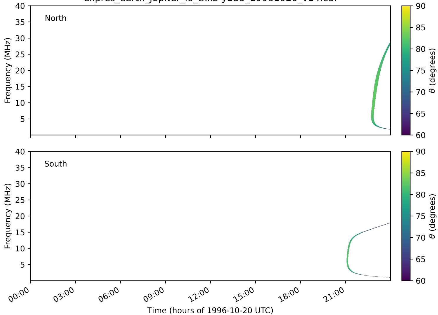
expres_earth_jupiter_io_txka-y235_19961020_v14.cdf
