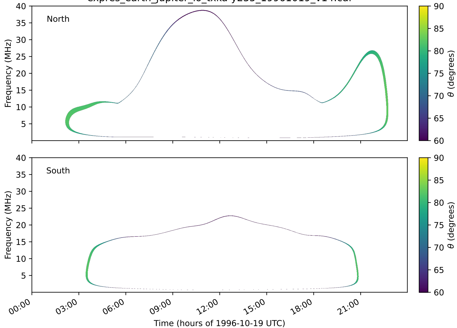
expres_earth_jupiter_io_txka-y235_19961019_v14.cdf
