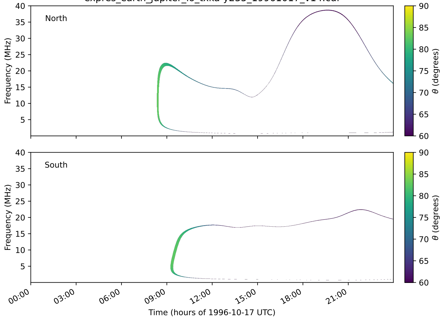
expres_earth_jupiter_io_txka-y235_19961017_v14.cdf
