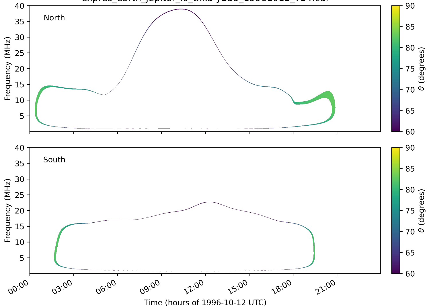
expres_earth_jupiter_io_txka-y235_19961012_v14.cdf
