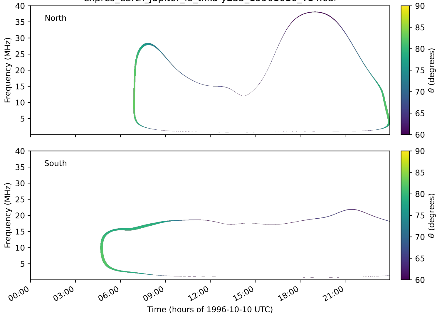
expres_earth_jupiter_io_txka-y235_19961010_v14.cdf
