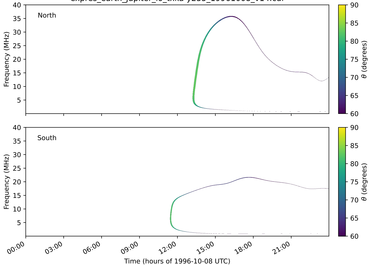
expres_earth_jupiter_io_txka-y235_19961008_v14.cdf
