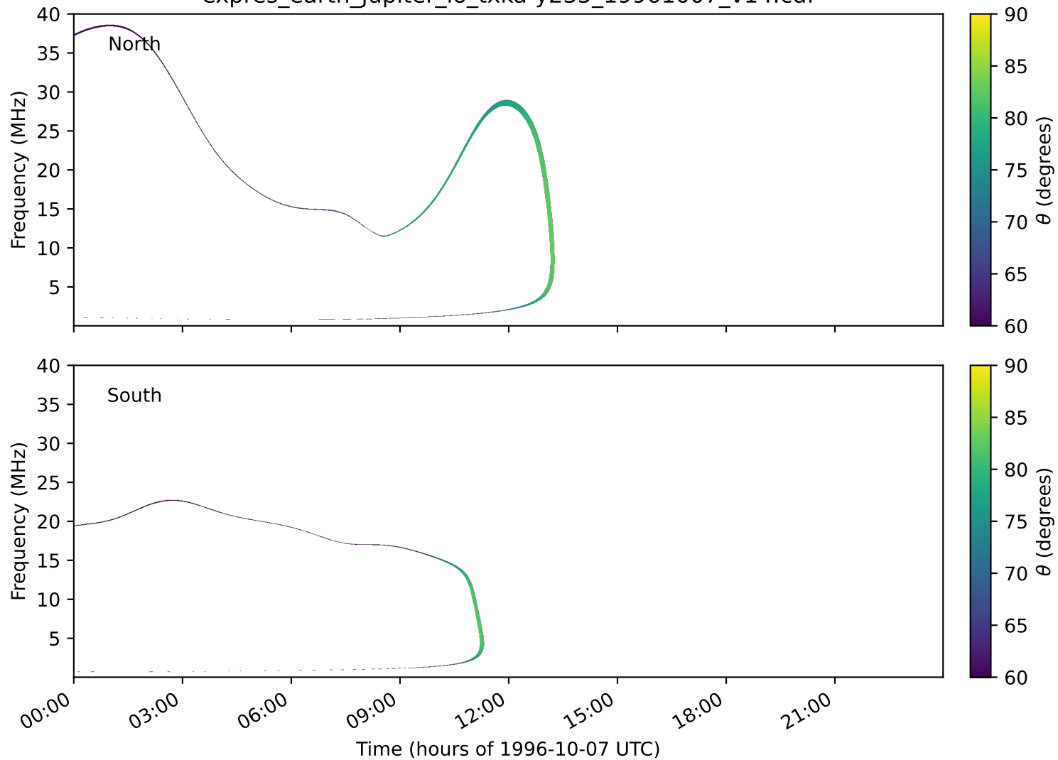
expres_earth_jupiter_io_txka-y235_19961007_v14.cdf
