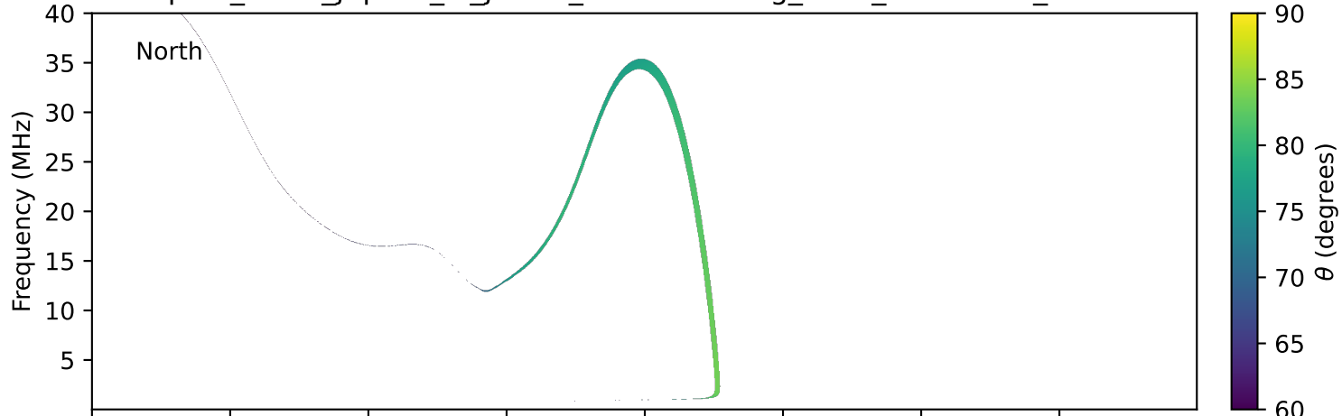
expres_earth_jupiter_io_jrm33_lossc-wid1deg_3kev_19961007_v11.cdf
