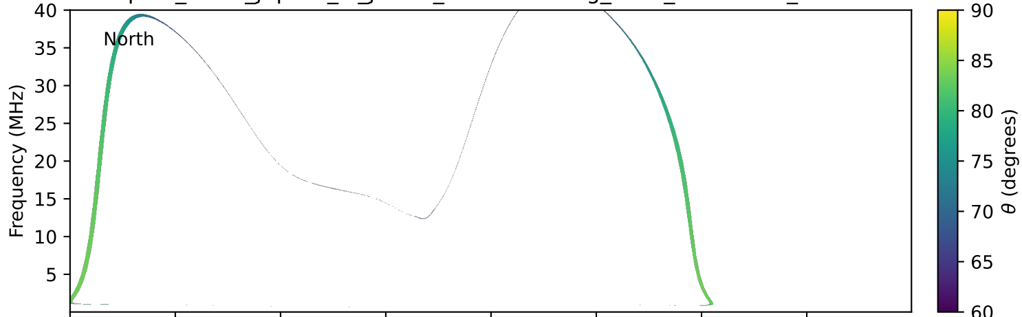
expres_earth_jupiter_io_jrm09_lossc-wid1deg_3kev_19961028_v11.cdf
