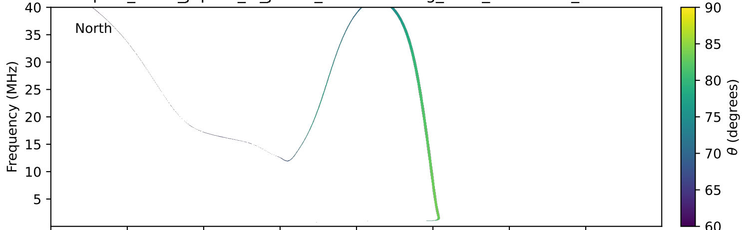
expres_earth_jupiter_io_jrm09_lossc-wid1deg_3kev_19961014_v11.cdf
