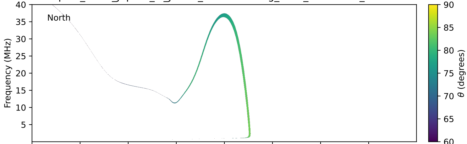
expres_earth_jupiter_io_jrm09_lossc-wid1deg_3kev_19961007_v11.cdf
