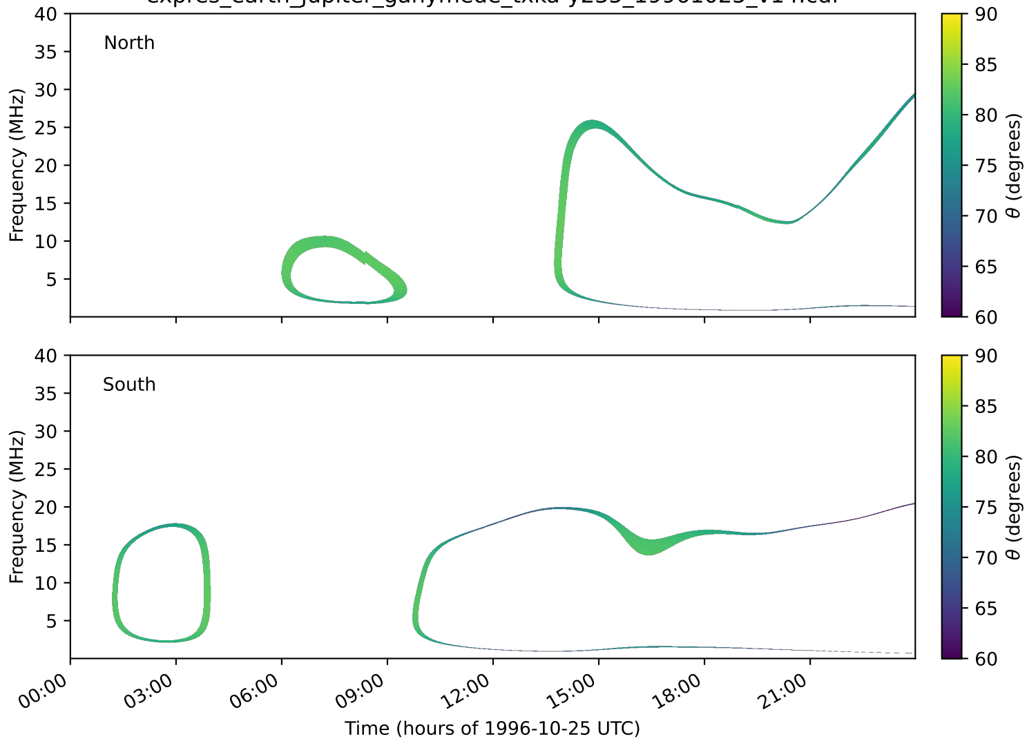
expres_earth_jupiter_ganymede_txka-y235_19961025_v14.cdf
