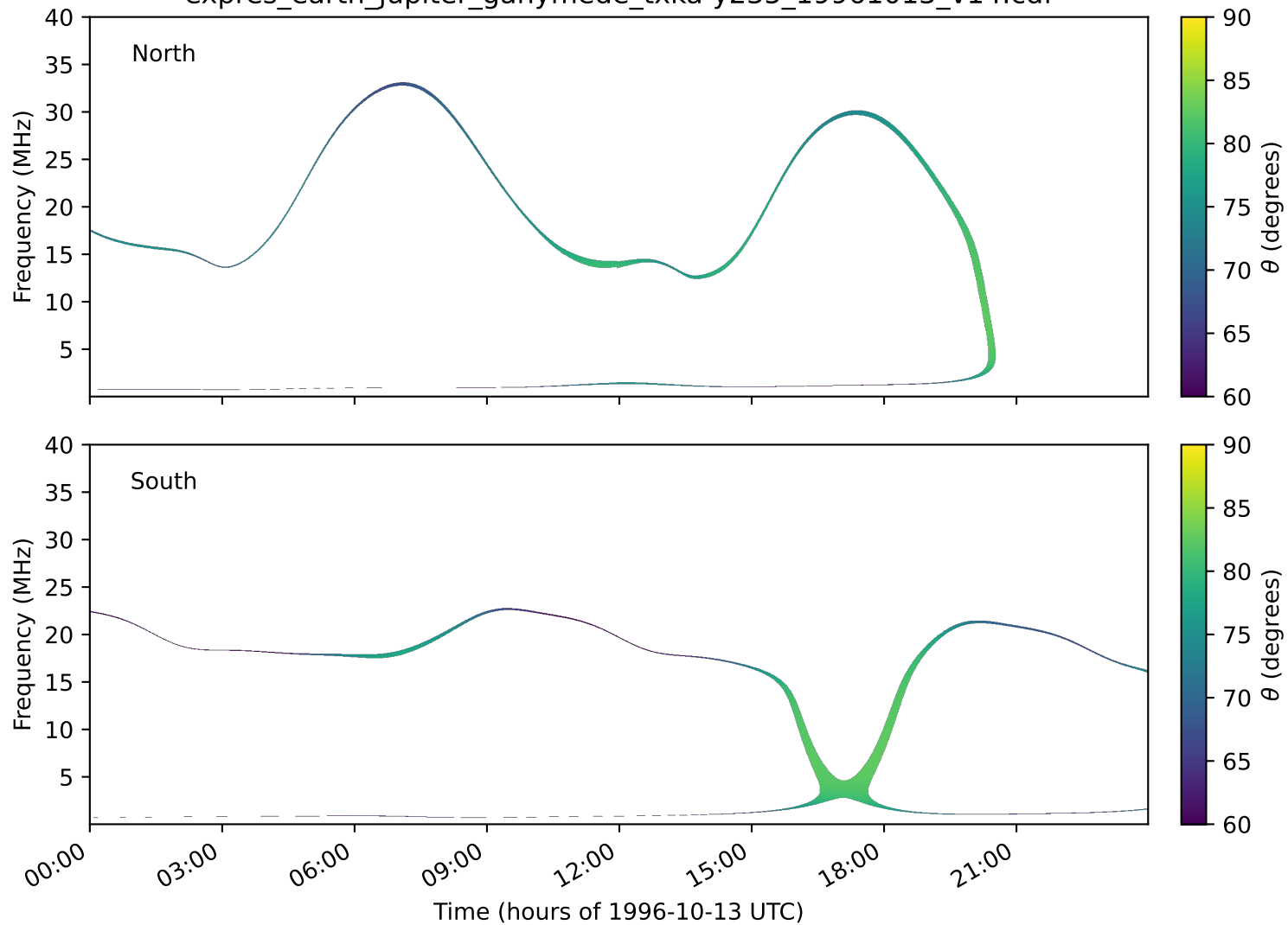
expres_earth_jupiter_ganymede_txka-y235_19961013_v14.cdf
