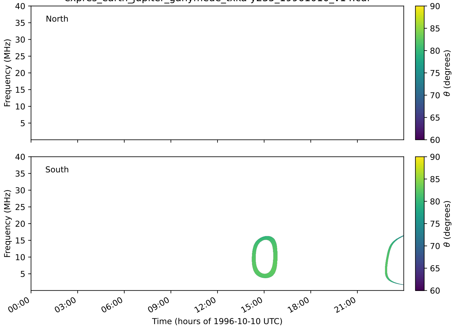
expres_earth_jupiter_ganymede_txka-y235_19961010_v14.cdf
