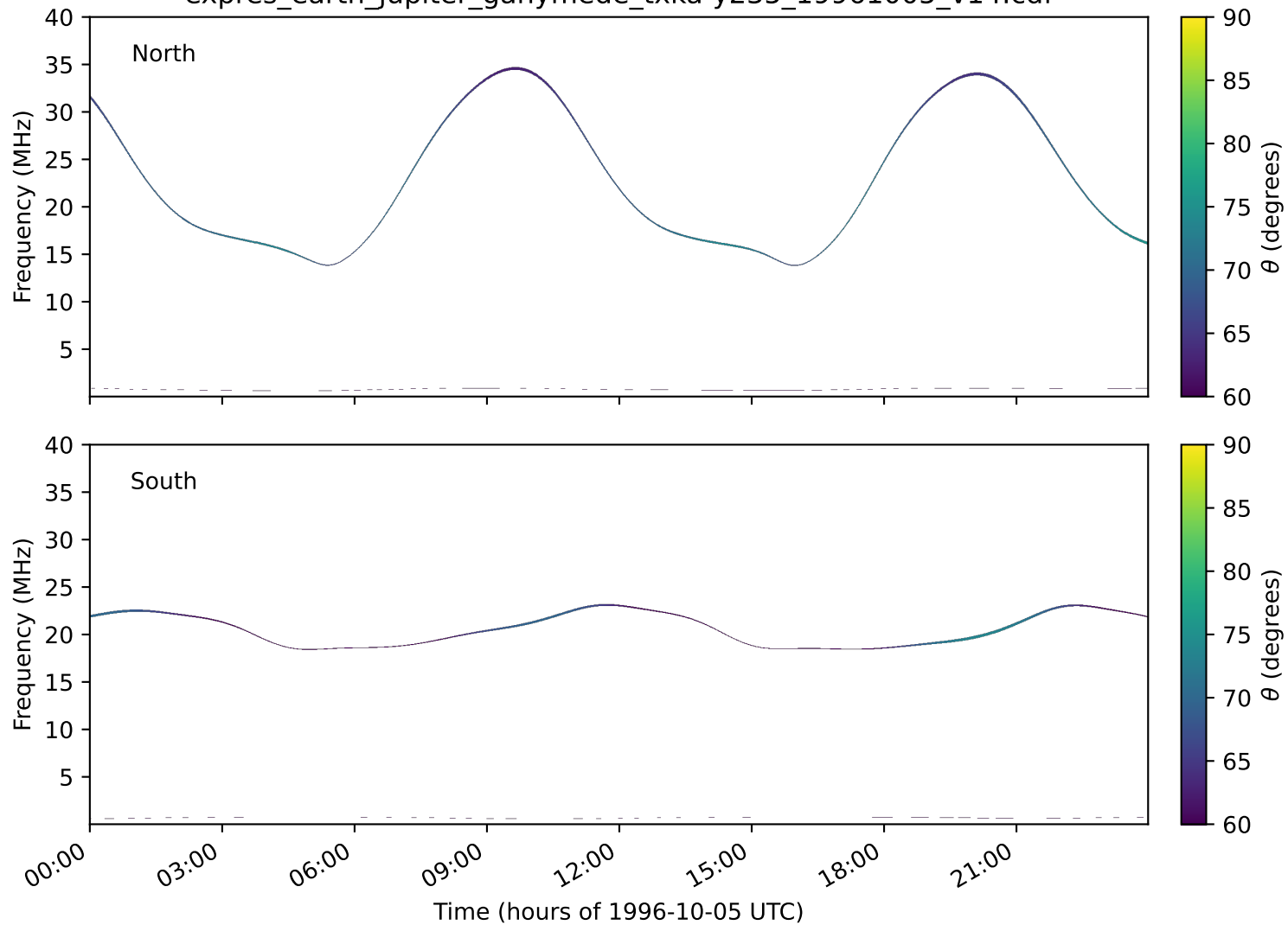
expres_earth_jupiter_ganymede_txka-y235_19961005_v14.cdf
