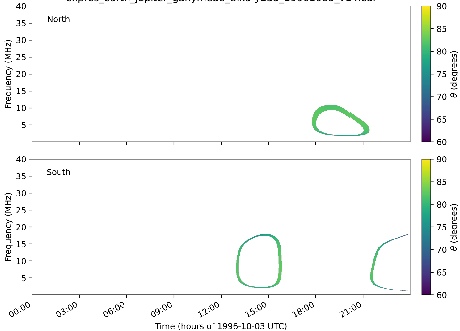
expres_earth_jupiter_ganymede_txka-y235_19961003_v14.cdf
