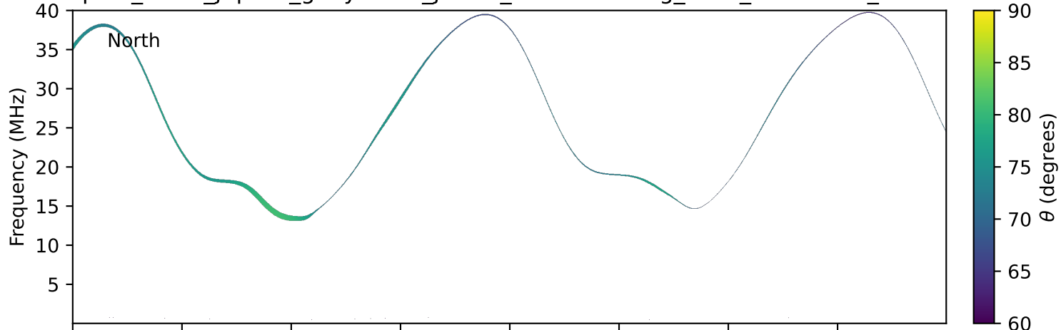
expres_earth_jupiter_ganymede_jrm33_lossc-wid1deg_3kev_19961026_v11.cdf
