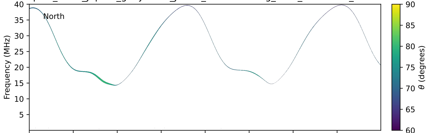
expres_earth_jupiter_ganymede_jrm33_lossc-wid1deg_3kev_19961019_v11.cdf
