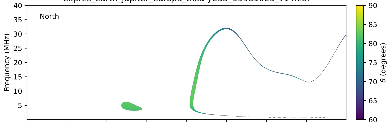
expres_earth_jupiter_europa_txka-y235_19961025_v14.cdf
