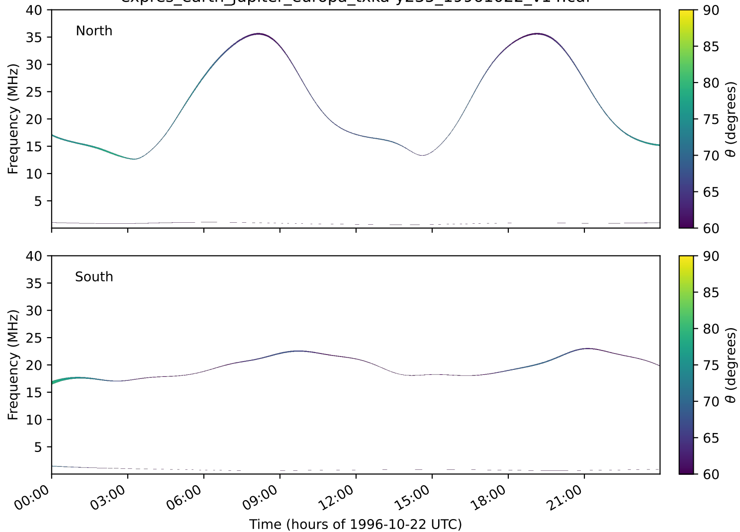
expres_earth_jupiter_europa_txka-y235_19961022_v14.cdf
