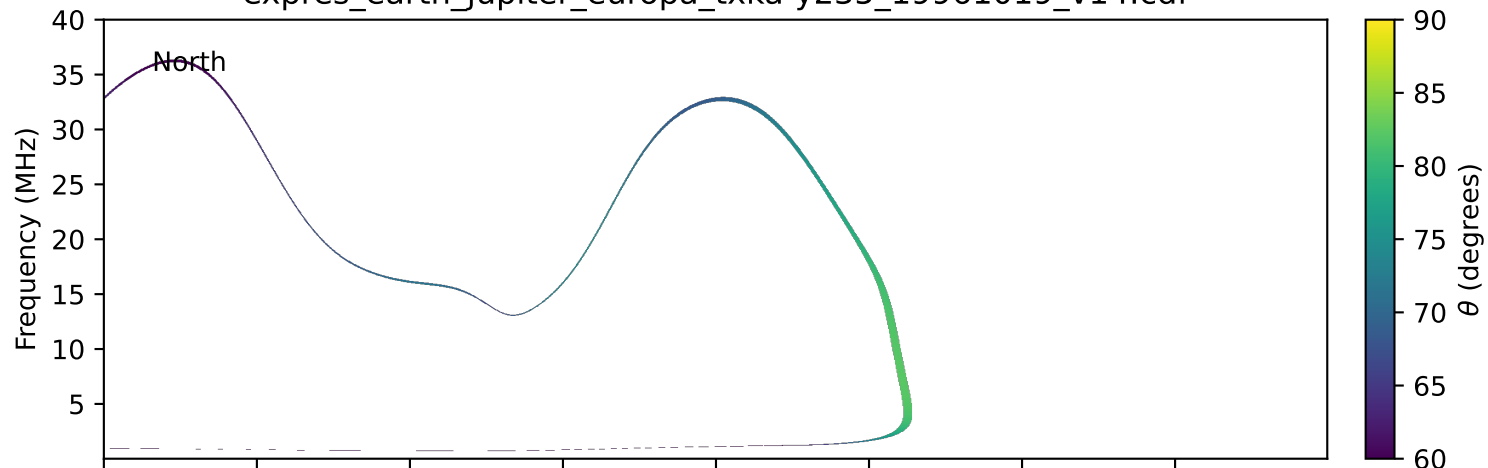
expres_earth_jupiter_europa_txka-y235_19961019_v14.cdf
