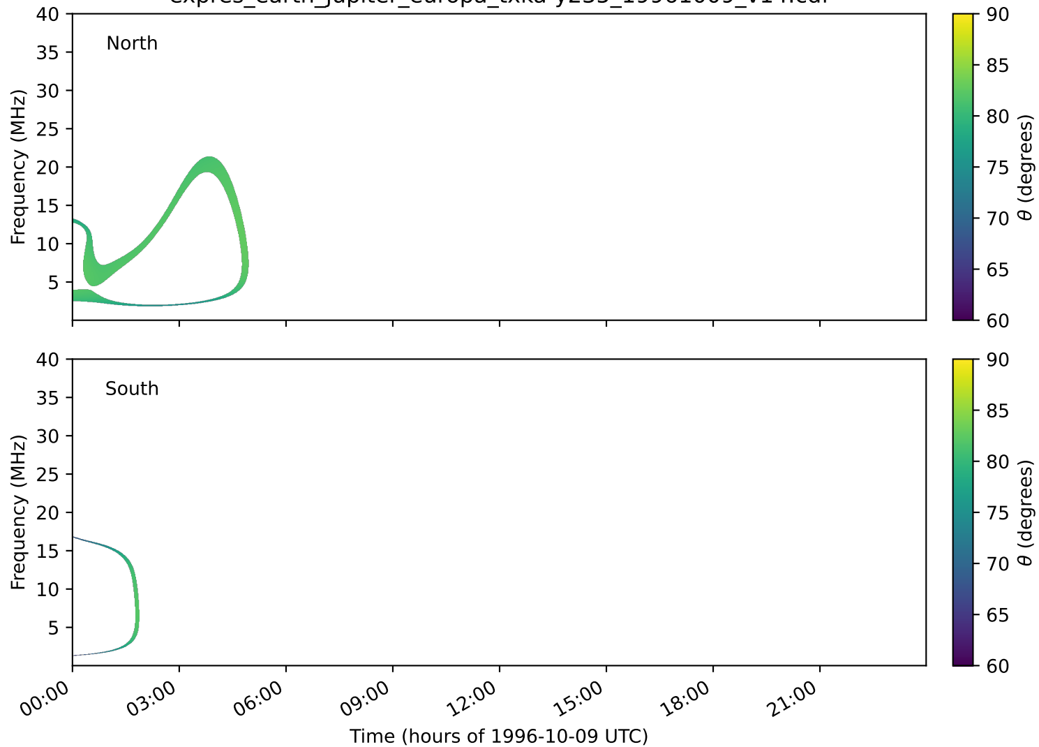
expres_earth_jupiter_europa_txka-y235_19961009_v14.cdf
